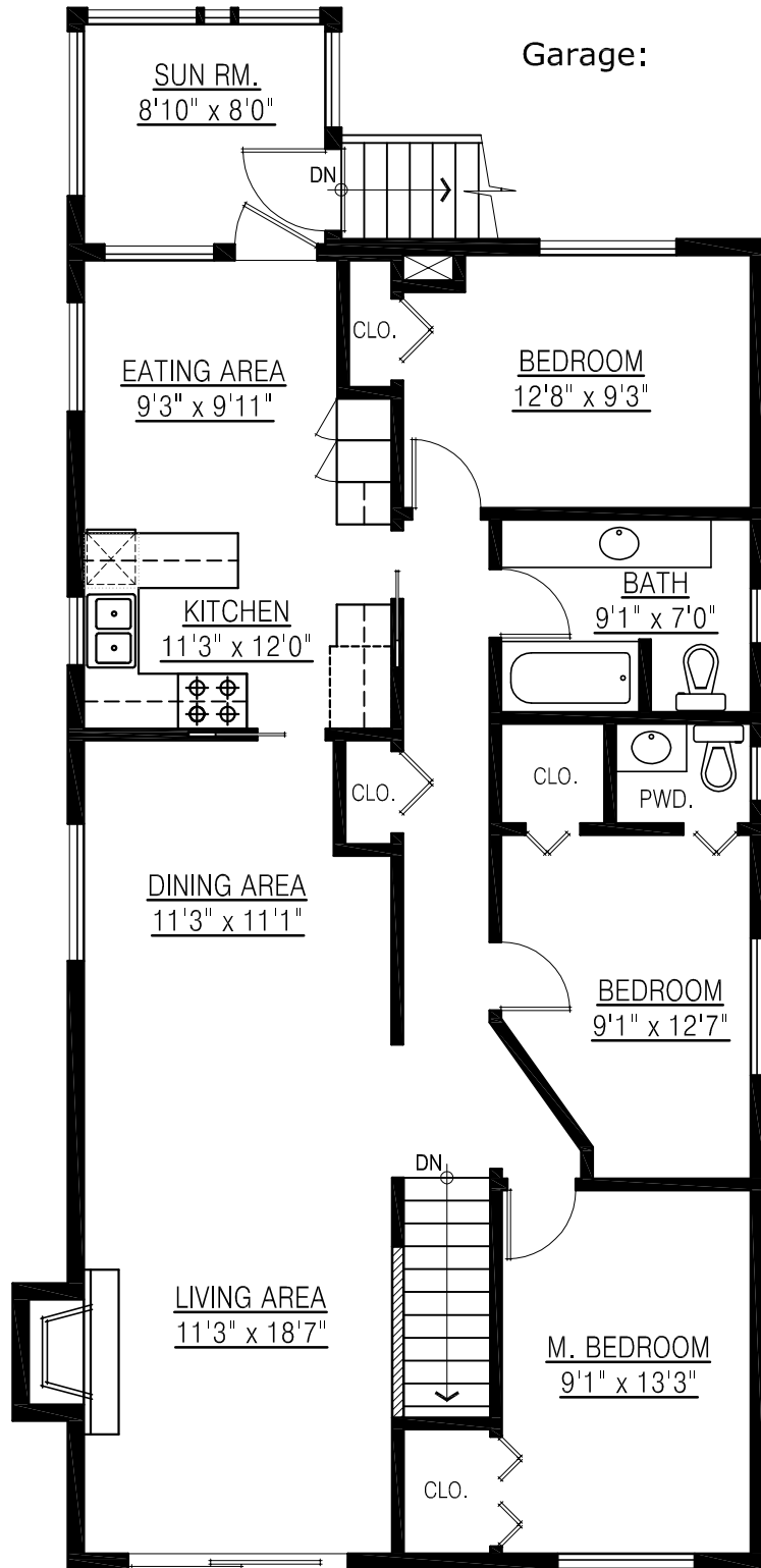
UPPER FLOOR PLAN FLOOR AREA: 1,310 sq.ft.
