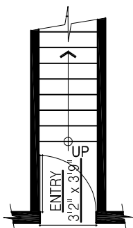
MAIN FLOOR PLAN FLOOR AREA: 32 sq.ft.
